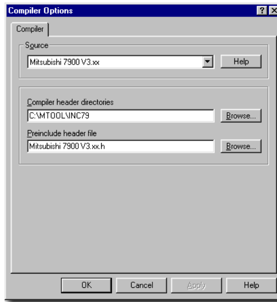
Figure 2.6 Compiler Options
