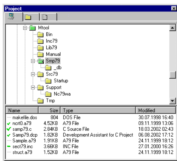
Figure 2.7 Project Window - Explorer View (Undocked mode)
