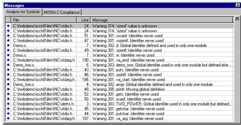
Figure 2.8 Messages Window - Analysis for Symbols tab (Undocked mode)
